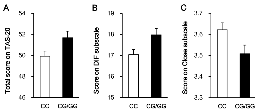
Fig re 1 Effects of 5-HTT C 1019G polymorphism on alexithymia and close attachment orientation. (A) Individuals with the CC genotype ( n = 316 ) had a lower mean total score on the 20 item Toronto Alexithymia Scale (TAS 20) than individuals with the CG/GG genotypes ( n = 188 ). (B) Individuals with the CC genotype reported a lower mean total score on the Difficulty Identifying Feelings (DIF) subscale of TAS 20 than individuals with the CG/GG genotype. (C) Individuals with the CC genotype reported a higher mean score on the close subscale of Revised Adult Attachment Scale than individuals with the CG/GG genotype. Standard errors of the means are shown as error bars.
